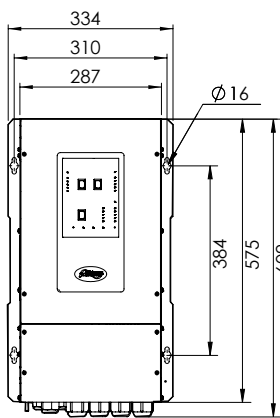
Front view 24 | 4000 24 | 7000
