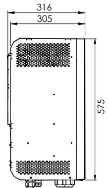
Side view 24 | 14000
