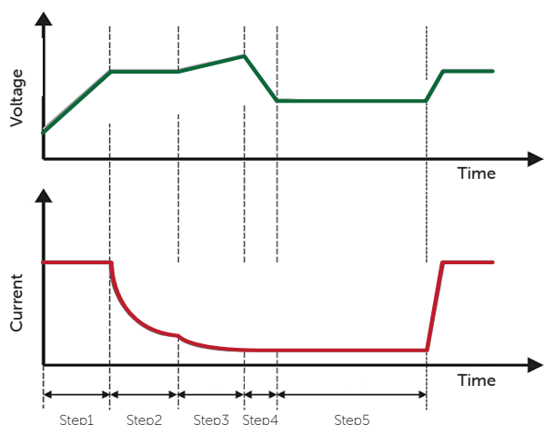
Graph illustrating multi-step charge algorithm
