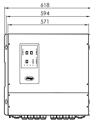
Front view 24 | 14000
